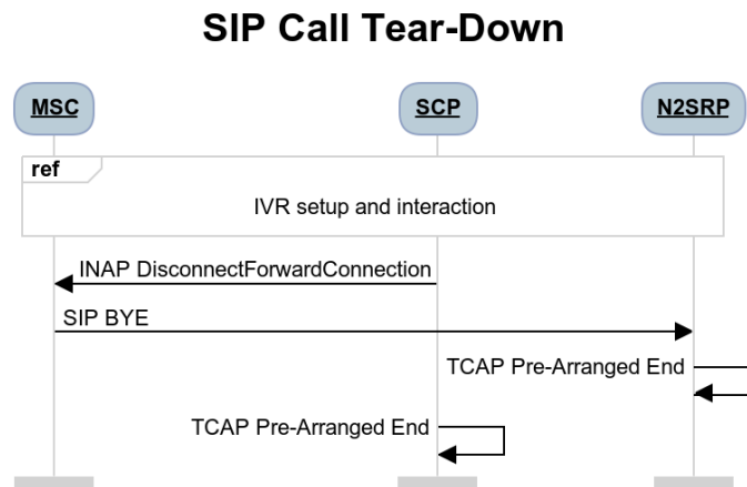
Figure E: SIP INAP Call Tear-Down (BYE from MSC)
